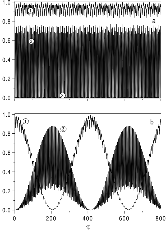
FIG. 1. Populations vs. \tau = \omega_L t for an ammonia molecule initially prepared in: (a) the |0^+ \rangle state; and (b) the |0^- \rangle state. Curves (1) give the total population of the lower doublet; curve (2) gives the population of the |0^- \rangle state; and curves (3) give the population of the upper level |3^+ \rangle .
